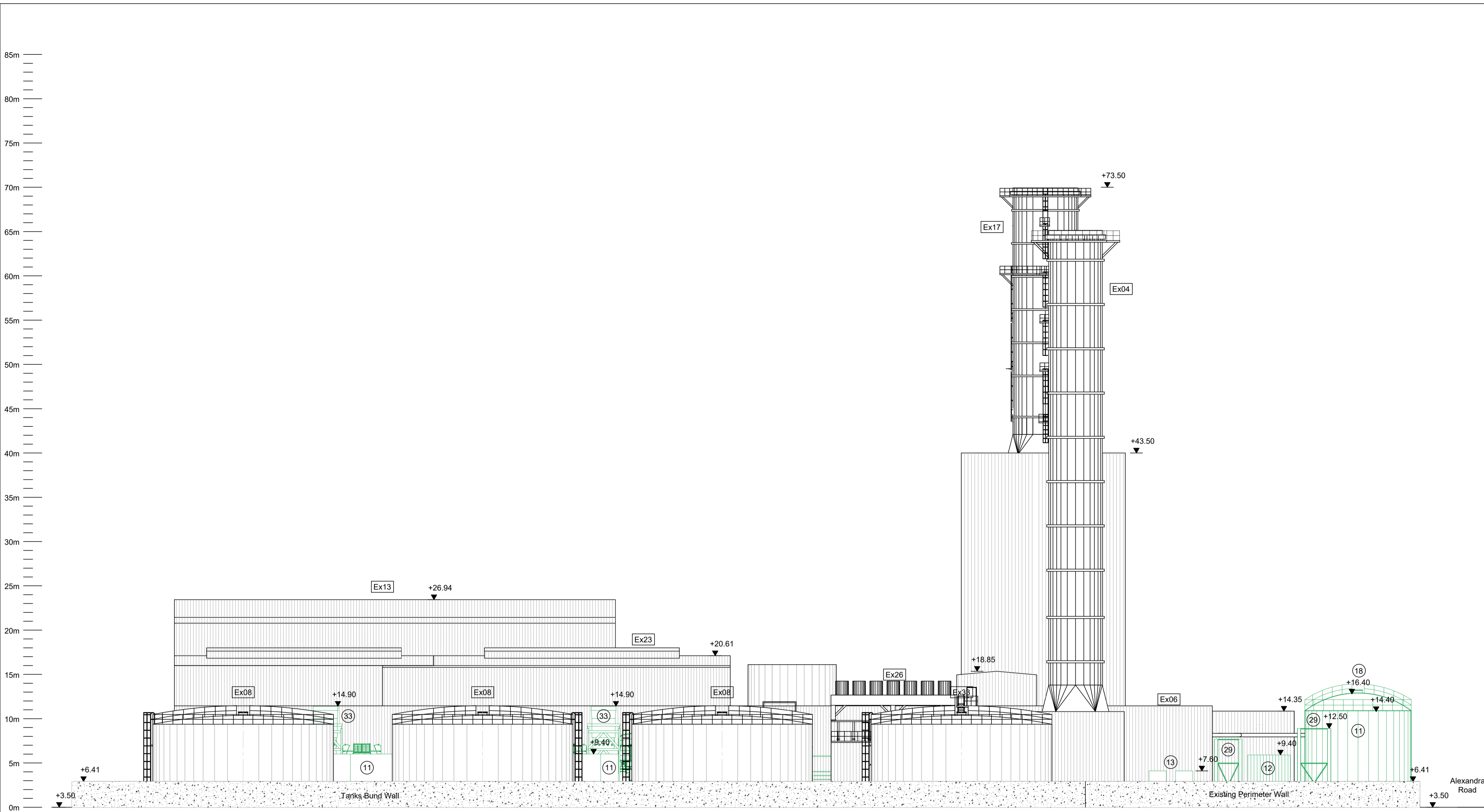
East Elevation 1:250
